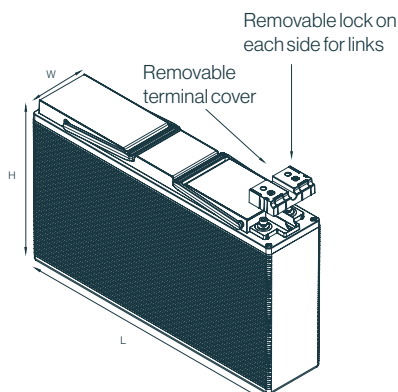
170FT with standard M8 terminal
