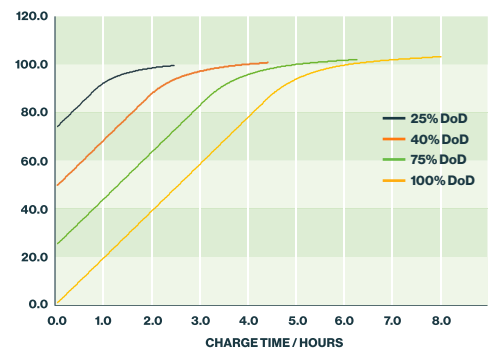
Recharge curves 2.400PC 2x110
