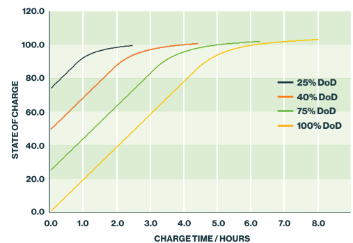
Recharge curves 2.400PC 2x110
