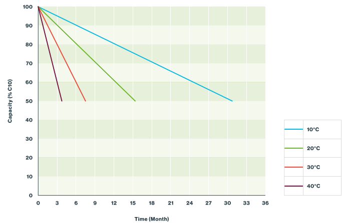
Self discharge
