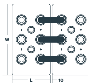
14 OPzS-ET1750 to 18 OPzS-ET2250
