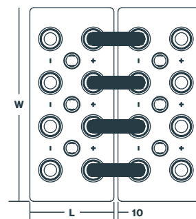
19 OPzS-ET2375 to 26 OPzS-ET3250
